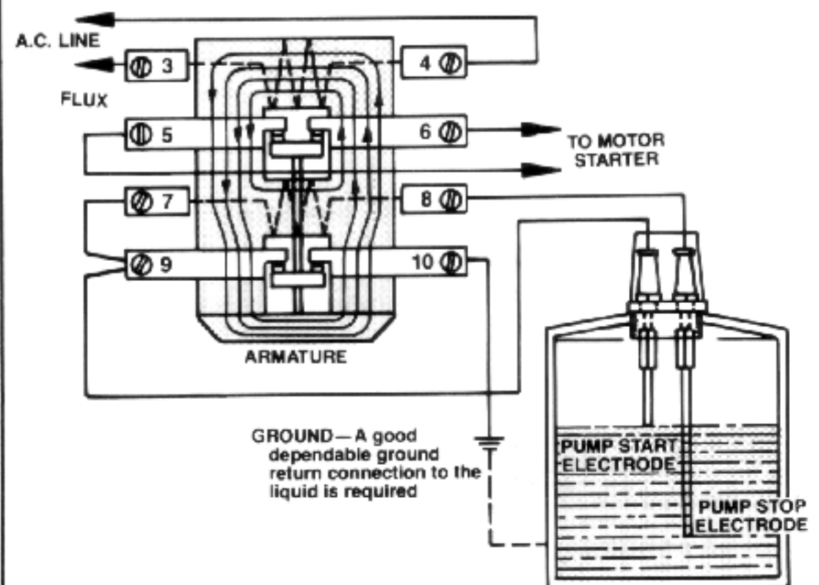
Figure 2—Secondary coil circuit closed; armature up.
