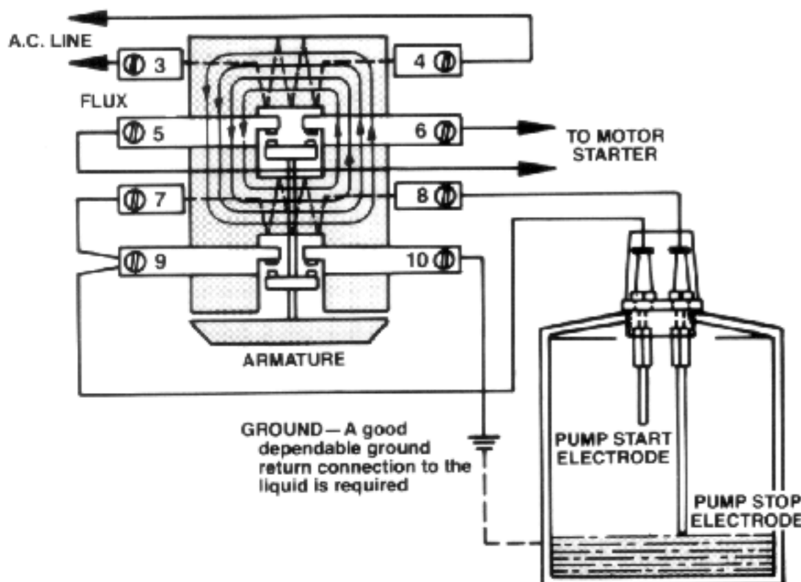
Figure 1—Secondary coil circuit open; armature down.
