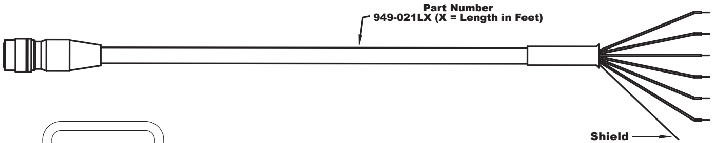
Figure 3.6 Wiring Diagram
