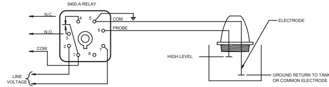
DIAGRAM C: HIGH LEVEL ALARM 5400-A DIRECT OPERATION 5400-A RELAY
