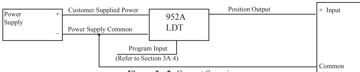
Figure 3 - 2: Current Sourcing
