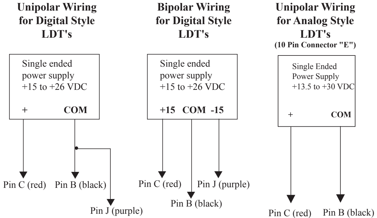
Figure 3-1: Power Supply Wiring (Unipolar/Bipolar)
