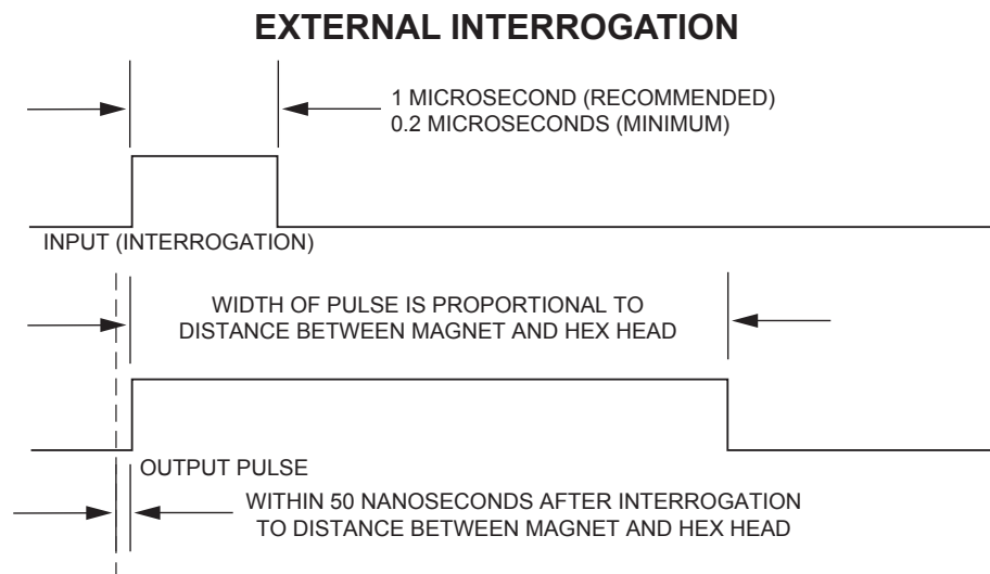
Figure 3-4: 952VP with External Interrogation
