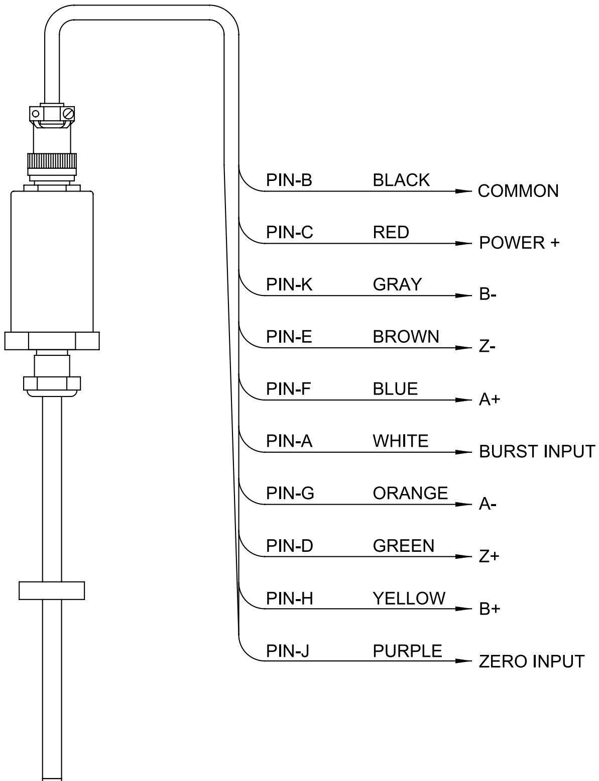
Figure 4-2: Wiring Diagram Drawing E0237900
