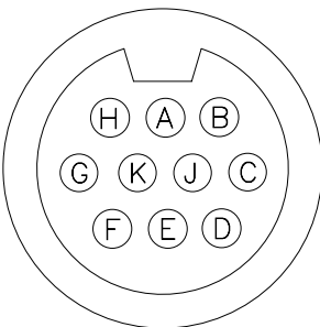
LDT Connector View MTS® Connector Option "RB" & "RC"
