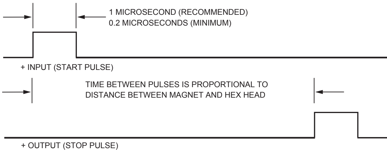
Figure 3-3: 952CP Control Pulse
