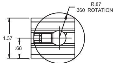
SLIDE MAGNET ASSEMBLY P/N SD0521800
