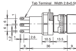
Solder/Tab Terminal
