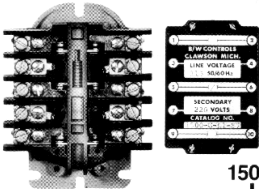
Cat. No. 1500-G-L1-S7 Shown with cover removed
