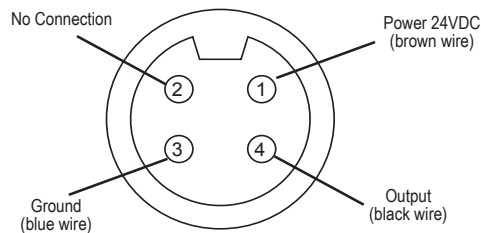
Connector View
