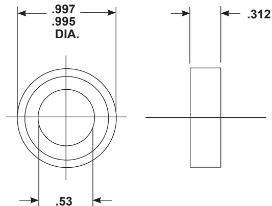
Cylinder Magnet
