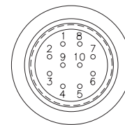
10 PIN HIROSE CONNECTOR VIEW
