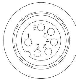
6 PIN CONNECTOR Connector View
