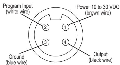
Connector View
