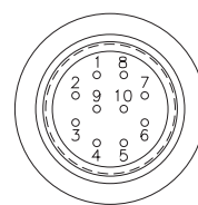
10 PIN HIROSE CONNECTOR VIEW
