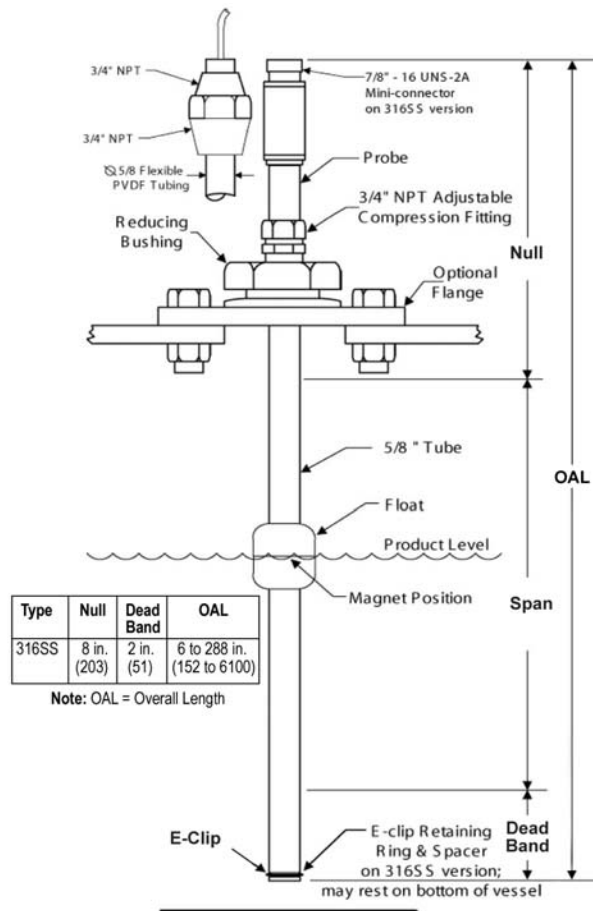
Typical Installation
