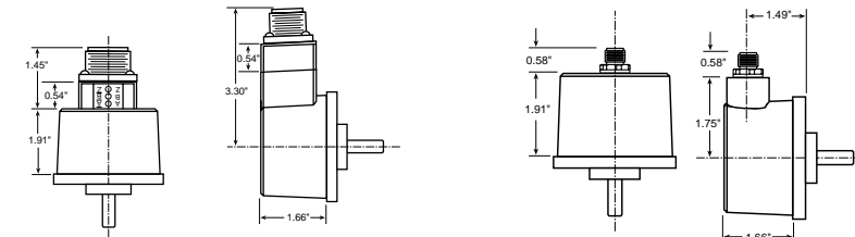
Code 6: 0 & 1 dimensions shown with LED Output Indicator Option (Code 7: PS)
