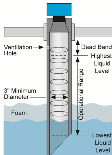
Stand-Pipe Mounting
