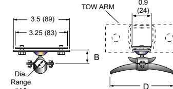
TOW CLAMP
