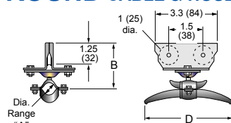
STEEL TROLLEY
