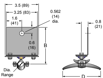
END CLAMP
