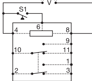
2. DPDT 11 Pin
