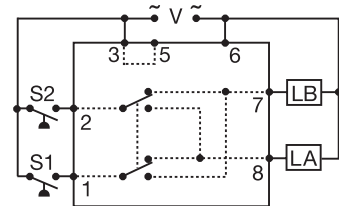
3. DPDT 8 Pin Cross Wired
