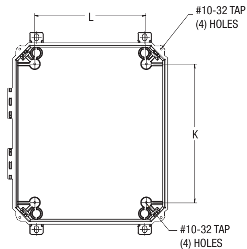
COVER REMOVED
