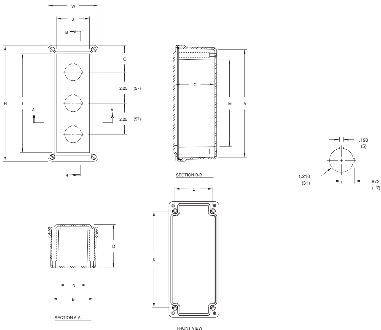
Pushbutton Series Enclosures - “30mm In-Line” Configuration Dimensions
