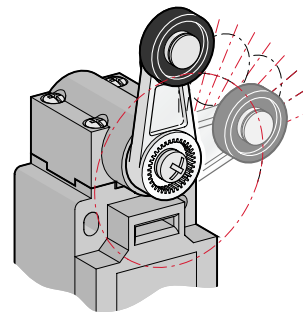
Free position adjustment 9 in 9° of lever: LS45P
